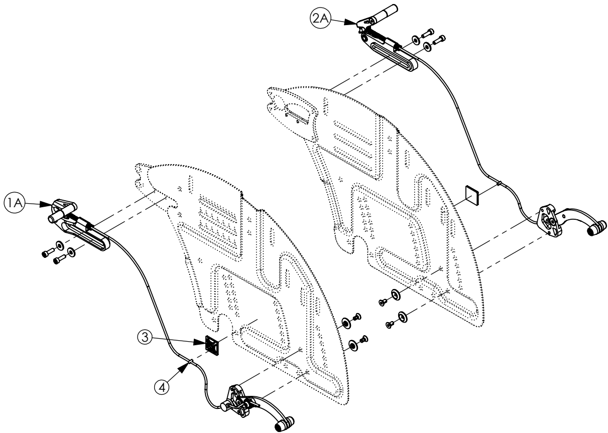
WHEEL LOCKS SHOWN IN FORWARD MOUNTING POSITION
